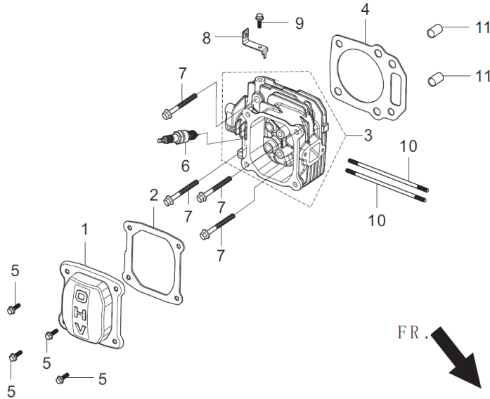
FIG.1 HEAD SUBASSEMBLY, CYLINDER / PLUG, SPARK (E04)
